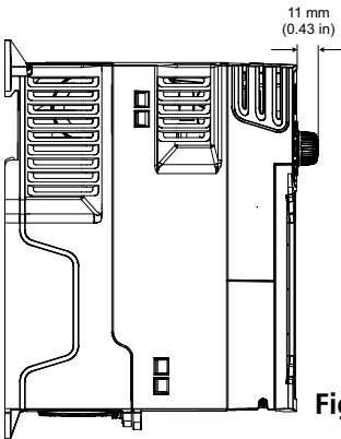
To accommodate the added depth with a potentiometer, add 0.43 in (11 mm) to the depth of the M201 drives. See Fig. #1 above. For NEMA Kit dimensions see page 30.
