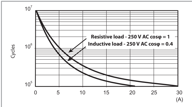
F 66-1 Electrical life (AC) v contact current - Type 66.82 250 V (normally open contact)
