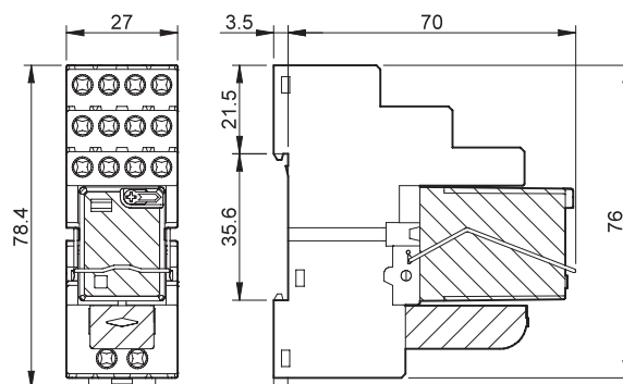
Type 58.P4 Push-in terminals
