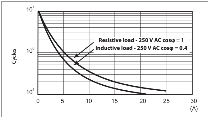
F 66-3 Electrical life (AC) v contact current - Type 66.22 250 V (normally open contact)
