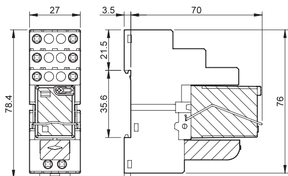
Type 58.P3 Push-in terminals
