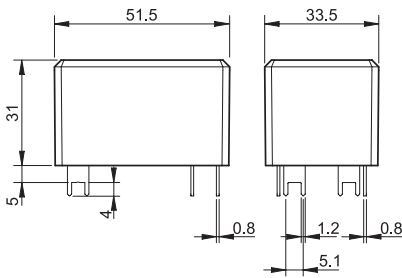
Type 66.22-xx03S/66.22-x603S
