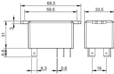
Type 66.82-x003
