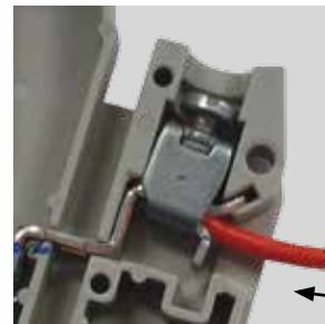
Screw terminal
