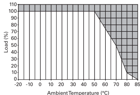
Vertical and Horizontal Mounting Position PSG240E24RM
