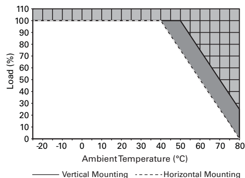
Vertical and Horizontal Mounting Position PSG240E24RM
